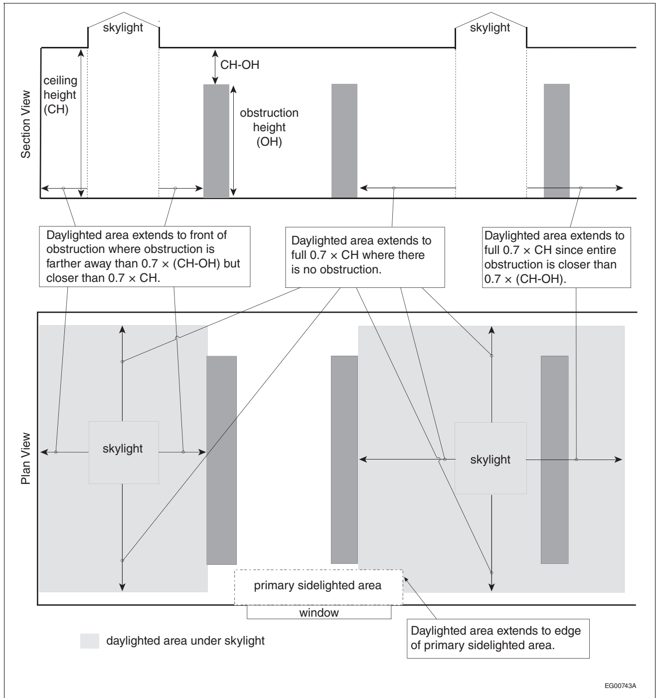
Figure A-4.2.2.5.(2) Determining daylighted area under skylights
